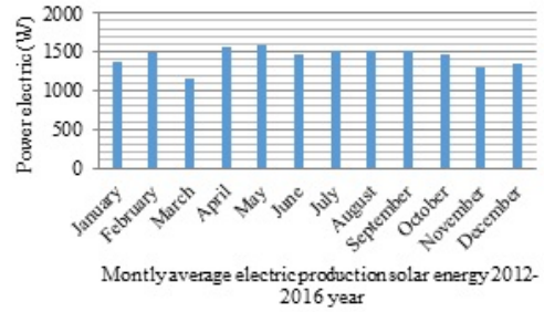
Fig. 6. Monthly production solar energy for 2012-2016
