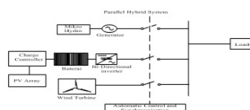
Fig. 1. The circuit diagram of the microgrid system
