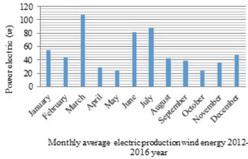
Fig. 4. Monthly electricity production from wind energy for 2012-2016
