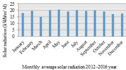
Fig. 5. Monthly solar radiation in the studied place for 2012-2016
